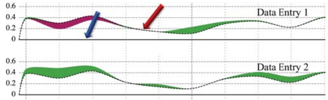
Fig. 6. The detail view in our MTSAD visualization of two example data entries. For instance, the solid line, at the blue arrow, is the base-line for the data entry (its position). The dashed line at the red arrow shows the outlying scores across the time of the multidimensional plots (the radar charts). The purple stream shows negative contributions, and the green one represents the positive contributions of the data entry to the overall outlying score of the multidimensional plots.
